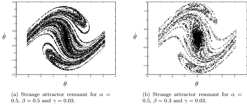
Figure 12: Strange attractor remnants for \alpha = 0.5 and \gamma = 0.03 .
