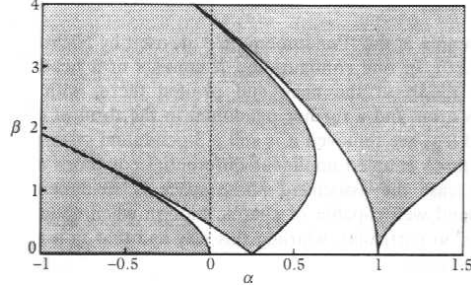
Figure 2: Stability diagram for Mathieu's equations (2.2,2.3). To the right of the dotted line ( \alpha = 0 ), the \theta = 0 state is unstable in the shaded region, on the left the \theta = \pi state is unstable in the shaded region. Only the region \beta \geq 0 is explicitly represented as the diagram is even in \beta .
