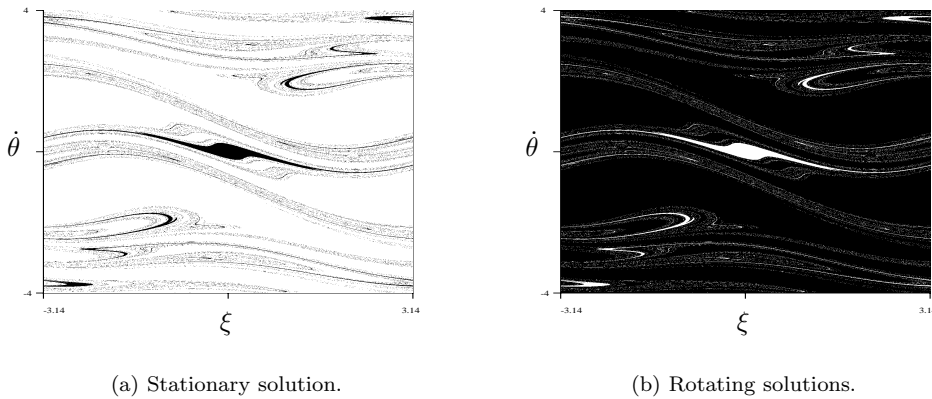
Figure 8: Coexistence of three basins of attraction (in black) for the vertically driven pendulum with \alpha = -0.1 , \beta = 0.545 and \gamma = 0.08 ; one has \xi = \pi + \theta .
