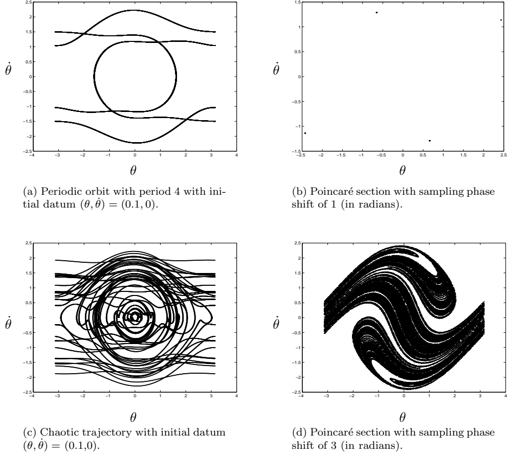
Figure 11: A chaotic trajectory and a periodic trajectory with the corresponding Poincaré sections for \alpha = 0.5 and \gamma = 0.03 . The values of \beta are respectively \beta = 0.70 and \beta = 0.63 . Transients are disregarded.
