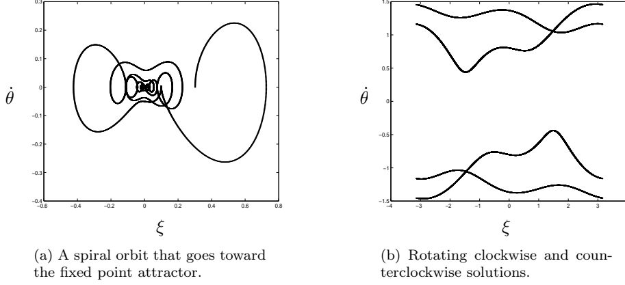
Figure 7: Attractors for the vertically driven pendulum with \alpha = -0.1 , \beta = 0.545 and \gamma = 0.08 .
