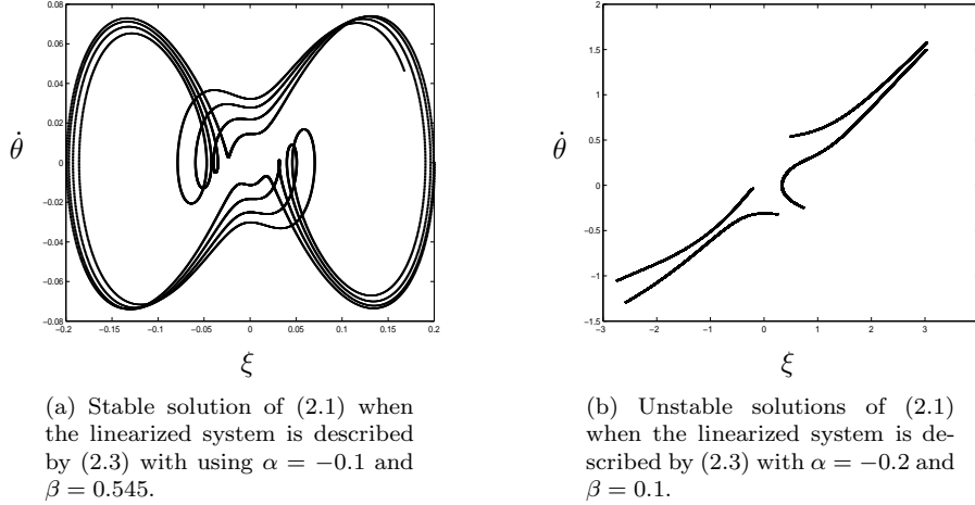
Figure 4: Stability and instability of the upward state of the pendulum described by (2.1).
