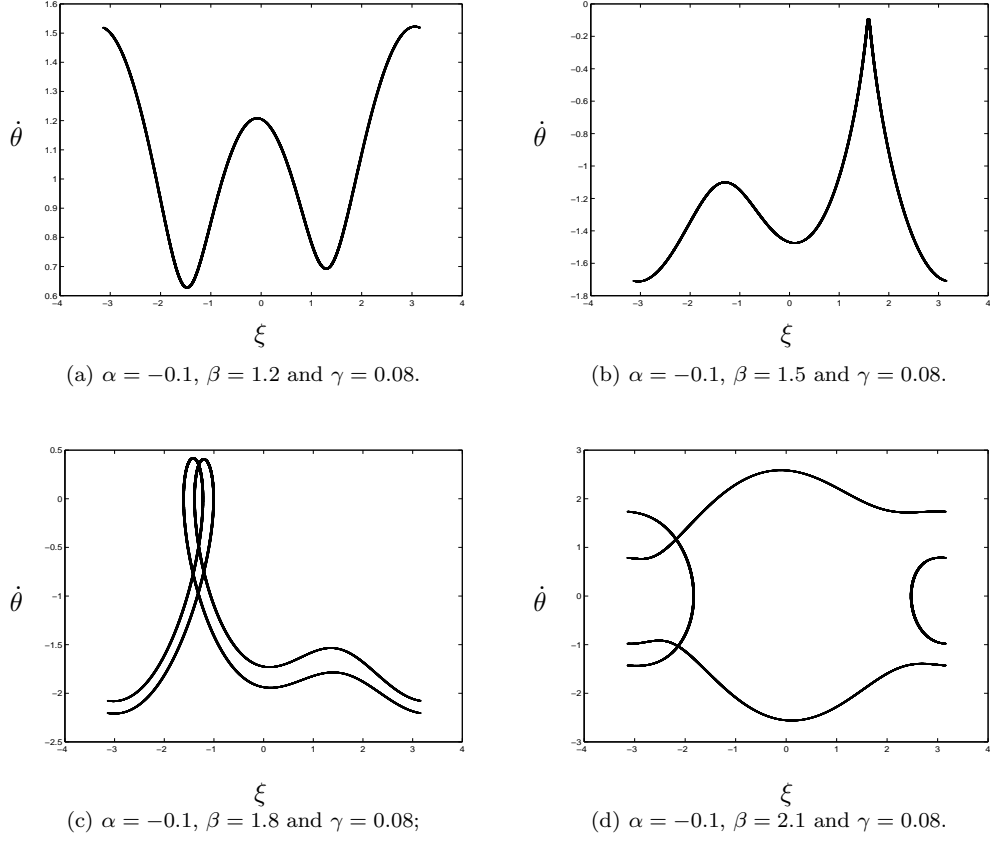
Figure 13: Smooth attractors (disregarding transients) for \alpha = -0.1 and \gamma = 0.08 .
