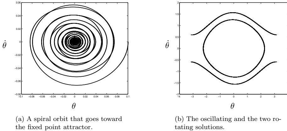
Figure 5: Attractors for the vertically driven pendulum with \alpha = 0.5, \beta = 0.1 and \gamma = 0.03 .
