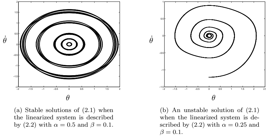
Figure 3: Stability and instability of the downward state of the pendulum described by (2.1).
