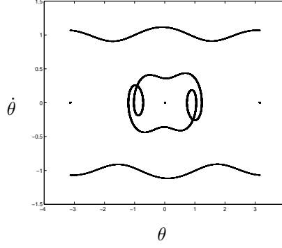
Figure 9: Attractors for the vertically driven pendulum with \alpha = 0.02 , \beta = 0.35 and \gamma = 0.03 .
