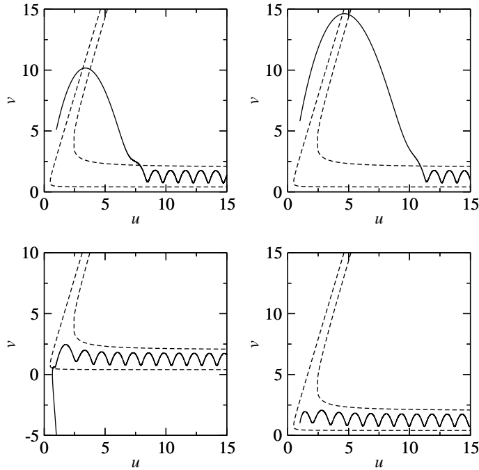
Figure 2: Numerically-obtained periodic solutions starting from various points in the u, v -plane, with f(t) = 3 + 2 \cos 2\pi t so f^+ = 5 , and parameters that satisfy the conditions of Theorem 1: m = 1 , u(0) = 1 , \gamma = 5 . The curves \Gamma^- and \Gamma^+ are shown dotted.
