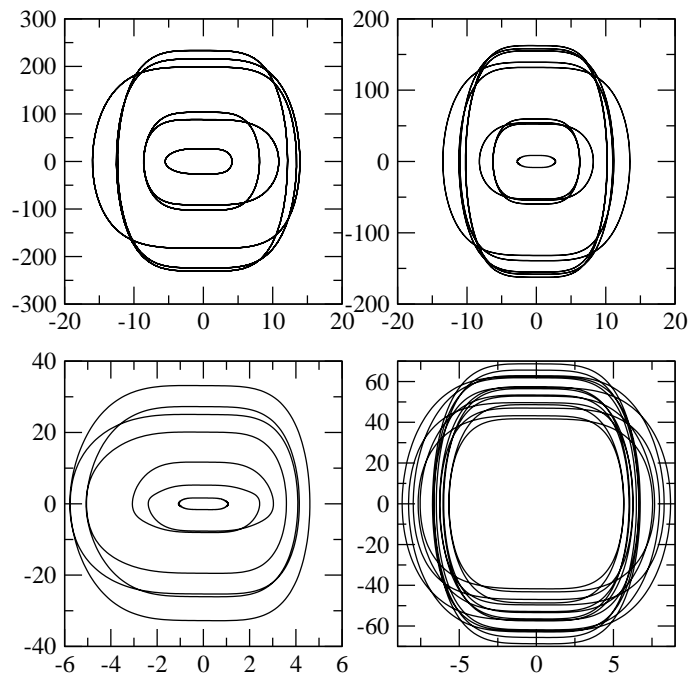
Figure 3: Numerical solutions to (1.1) with f(t) = 3 + 2 \cos 2\pi t and \gamma = 0.04 . In all four graphs, x is plotted horizontally and y vertically. The top left graph shows three period-one (same period as f(t) ) solutions; the top right graph shows three period-two solutions (repeating every two periods of f(t) ). Bottom left: three period-four solutions; bottom right, one period-ten solution.
