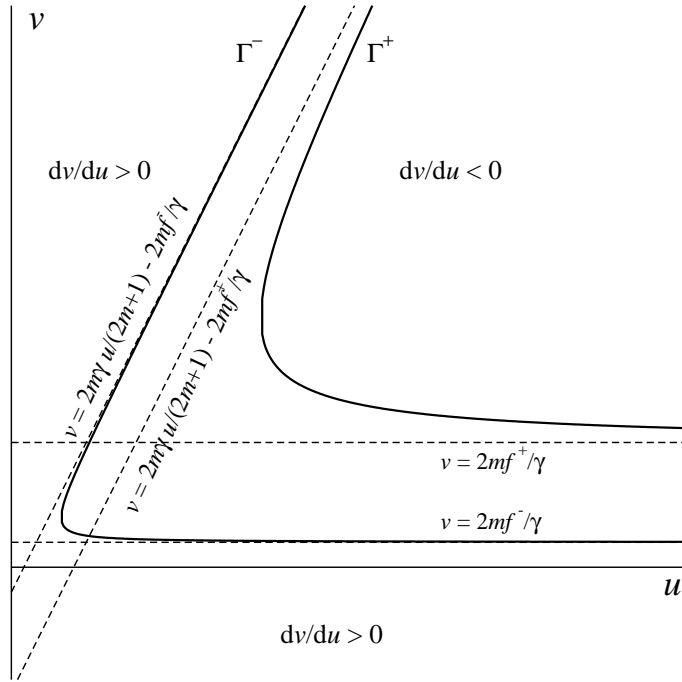
Figure 1: The curves \Gamma^+ and \Gamma^- and their asymptotes. To the left of \Gamma^- , dv/du is positive and to the right of \Gamma^+ it is negative. Between \Gamma^+ and \Gamma^- , dv/du can be positive, negative or zero.
