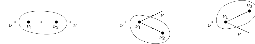
Figure 6: Self-energy clusters of order k = 2 with one line \ell and two nodes v_1 and v_2 with k_{v_1} = k_{v_2} = 1 : the exiting and entering lines have the same momentum, so that \nu_1 + \nu_2 = 0 , and the scale n_\ell of the line \ell is strictly smaller than the scales of both the exiting and entering lines (by definition of cluster).
