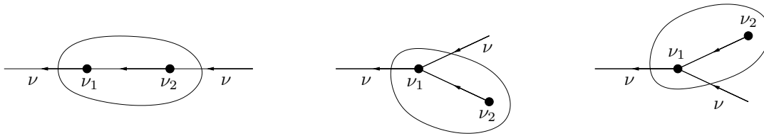
Figure 6: Self-energy clusters of order k = 2 with one line \ell and two nodes v_1 and v_2 with k_{v_1} = k_{v_2} = 1 : the exiting and entering lines have the same momentum, so that \nu_1 + \nu_2 = 0 , and the scale n_\ell of the line \ell is strictly smaller than the scales of both the exiting and entering lines (by definition of cluster).
