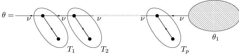
Figure 11: Example of tree with accumulation of small divisors for maximal tori.
