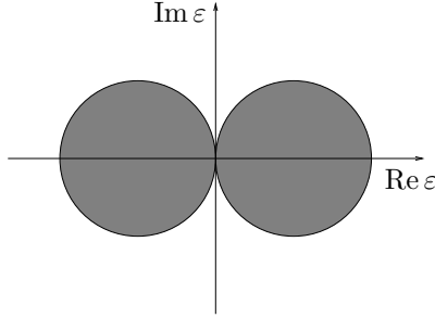
Figure 9: Analyticity domain for the response solution.
