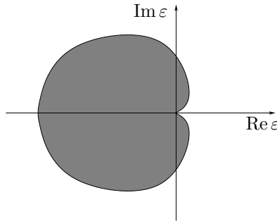
Figure 8: Analyticity domain for the hyperbolic invariant torus.
