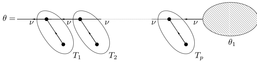
Figure 11: Example of tree with accumulation of small divisors for maximal tori.
