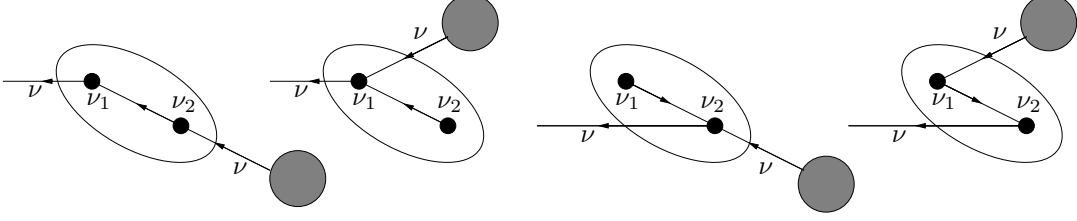
Figure 7: Cancellation up to second order in x of the values of the self-energy clusters of order k = 2 . In all self-energy clusters one has the same values of the mode labels \nu_1 and \nu_2 (with the constraint \nu_1 + \nu_2 = 0 ).
