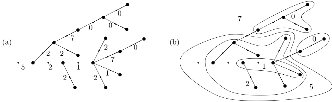
Figure 5: Example of clusters: in (a) a tree \theta is represented with the scale labels associated with its lines; in (b) the clusters corresponding to the same assignment of scale labels are drawn.
