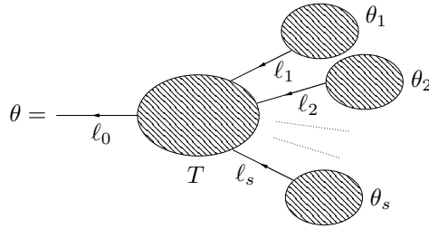
Figure 10: Construction for the proof of the Siegel-Bryuno lemma.
