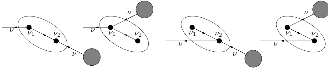
Figure 7: Cancellation up to second order in x of the values of the self-energy clusters of order k = 2 . In all self-energy clusters one has the same values of the mode labels \nu_1 and \nu_2 (with the constraint \nu_1 + \nu_2 = 0 ).
