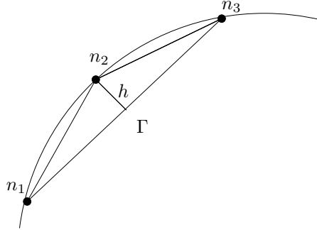
Figure 8. Simplex generated by three points n_1, n_2, n_3 on the sphere S^1(r) . \Gamma is the base of the spherical cap in which the three points are contained and h the height. If h is small then the volume (=area) of the cap is of order \Gamma^3/r , with \Gamma = O(|n_1 - n_2| + |n_1 - n_3|) .
